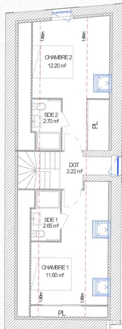
R+1
